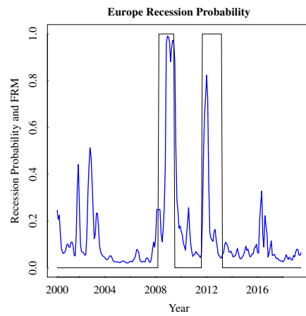
Fig. 16 The FRM-implied recession probability in the Europe The implied recession probability from the fitted logistic regression, and dated CEPR recession periods
