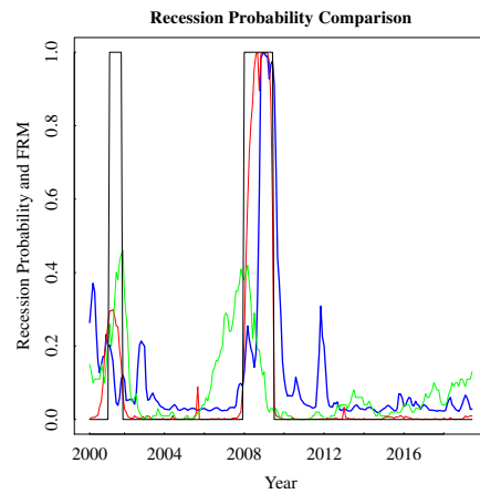
Fig. 17 The FRM-implied recession probability in comparison in the US NBER recession periods, FRM@Americas versus Smoothed US Recession Model , Yield Curve Slope Model
